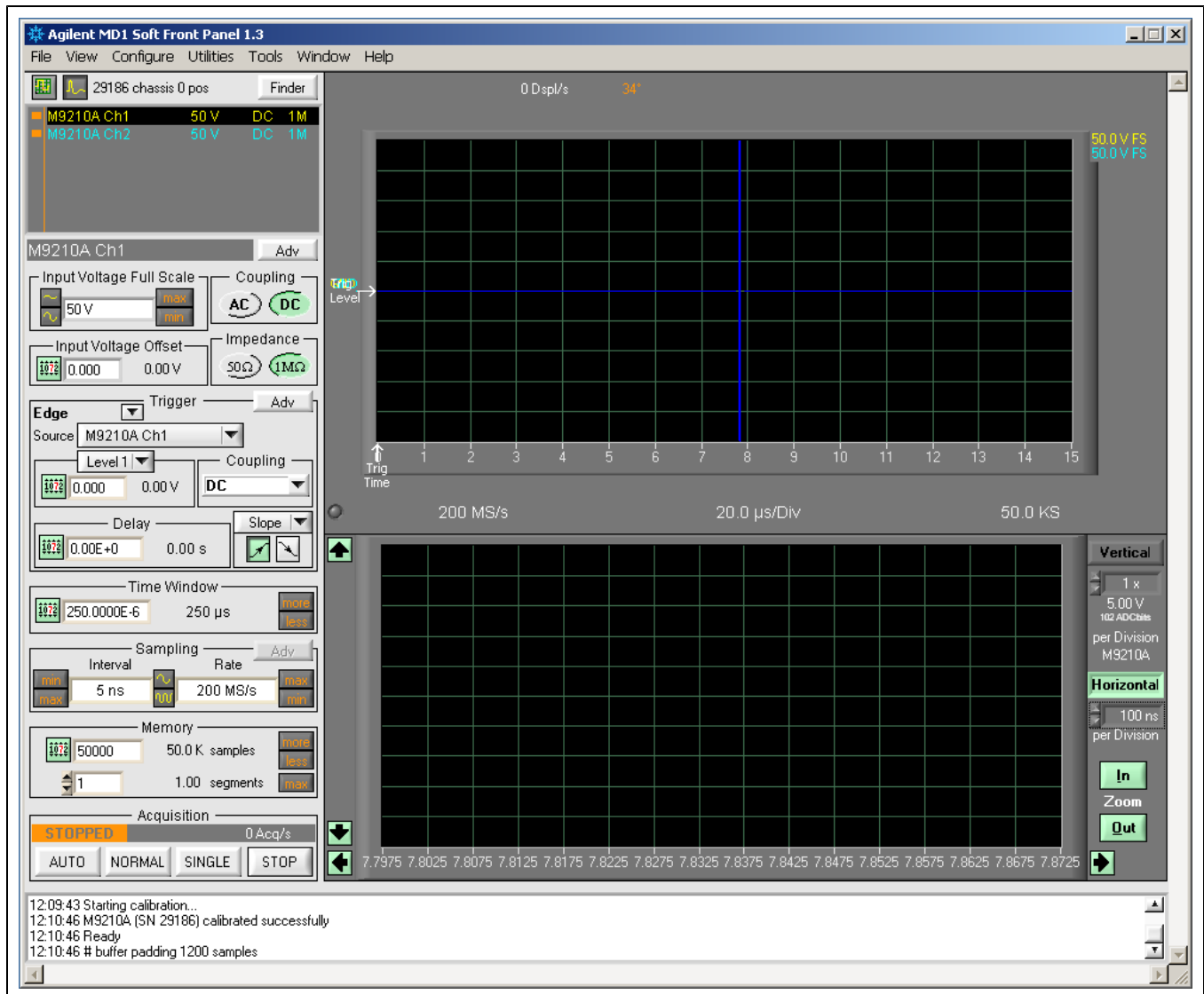
Figure 3 - Soft Front Panel (SFP) showing the result of the Self-Test
